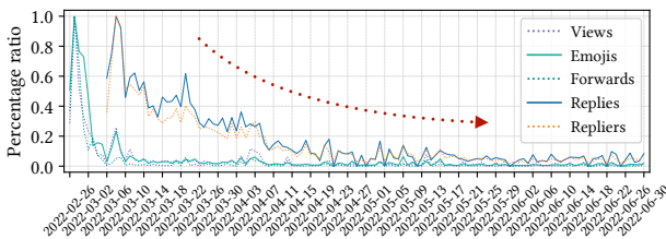
Figure 7: Levels of user engagement daily in the IT Army of Ukraine Telegram channel. Values are min-max normalised.
